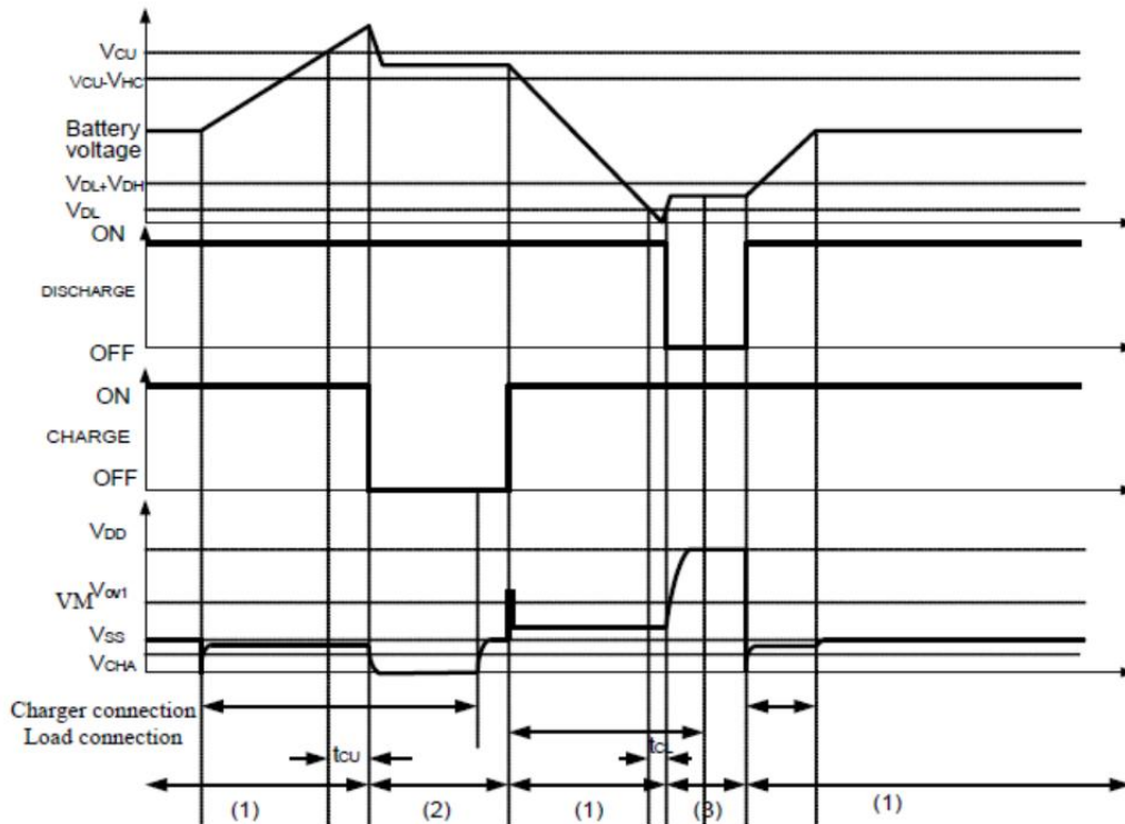
Figure5-1 Overcharge and Over discharge Voltage Detection
